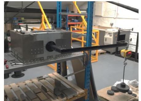
Figure 10 – Torque Testing Atlas Socket
