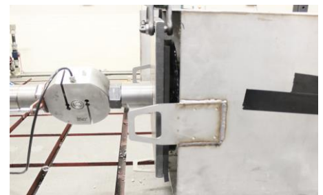
Figure 11 – Deflection Loading Testing
